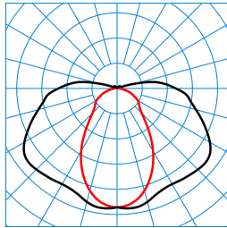
Acquex LED-M 1.5 80-840 ET PC EB3 TX774643
