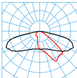
LIQ 50N-AB2L-LRA/4600-727 6G1 ETDD (CLO initial value) TX775211
