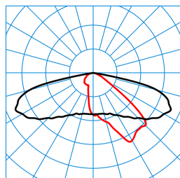
LIQ 50N-AB2L-LR/1200-740 2G1 ET (CLO initial value) TX775115
