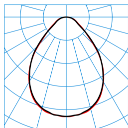
ArimoFit M46 PW19 42-8TW ETDD8 + ArimoFit Sky M46-TS ZER (DSU) TX874648
