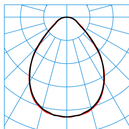
ArimoFit M46 PW19 42-8TW ETDD8 + ArimoFit Sky M46-TS ZER (DWW) TX874647
