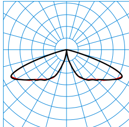
CS 19 C 100-RB6L/4200-730 4G1S ETDD (CLO end value) TX300168
