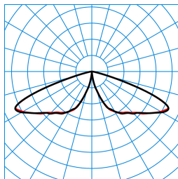
CS 19 C 100-RB6L/4200-730 4G1S ETDD (CLO initial value) TX300169
