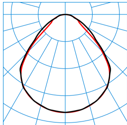
ValineoG4 M73 PW19 38-50/4ML-830 ET X2 (stage 1) TX773253
