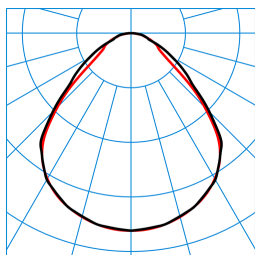
ValineoG4 M73 PW19 38-50/4ML-830 ET X2 (stage 3) TX773278
