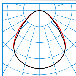
Siella G8 M84 PW19 28-40/3ML-8MC ET (stage 1) TX562675
