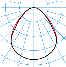
Siella G8 M84 PW19 28-40/3ML-8MC ET (stage 6) TX562625
