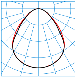
Siella G8 M84 PW19 28-40/3ML-8MC ET (stage 5) TX562713
