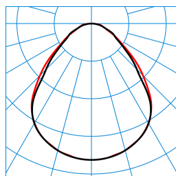
Siella G8 M84 PW19 28-40/3ML-8MC ET (stage 2) TX562615
