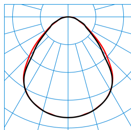
Siella G8 M84 PW19 28-40/3ML-8MC ET (stage 4) TX562605
