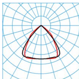
ELINE LW2240-110 ML 830 L150 2 20
