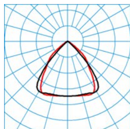
ELINE LW2240-110 ML 830 L150 4 20
