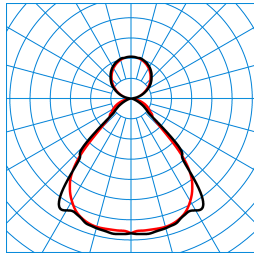
SFlow H2-L MRW LED6400-830 ET 03 TX721320
