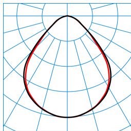
Opendo M39 PW19 42-840 ETBLE +CAS-S TX565206
