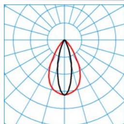
ELINE HE LEN40-120 ML 830 L150 0 20
