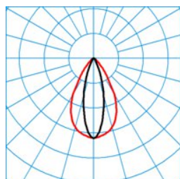
ELINE HE LEN40-120 ML 830 L150 4 20
