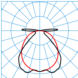
OleveonF 12 B 21-65/16 ML-840 PC (stage 4) TX194474
