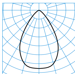
Amatris G4 C04 HR 14-20/3ML-840 ETDD 01 (stage 2) TX558419
