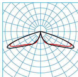
CS 19 100-RB6L/1200-730 2G1S ETDD (CLO initial value) TX300054
