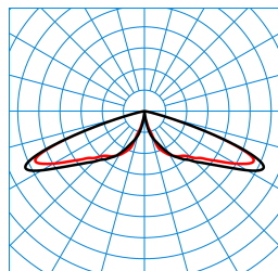
CS 19 100-RB6L/1200-730 2G1S ETDD (CLO end value) TX300053
