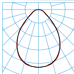
ArimoFit M46 PW19 42-830 ETDD + ArimoFit Sky M46-TS ZER TX426287
