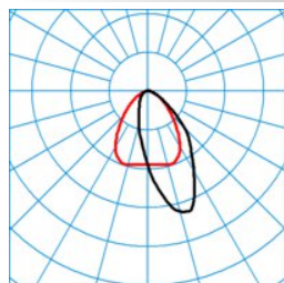
ELINE HE+ LAN120 865 L225 1 20
