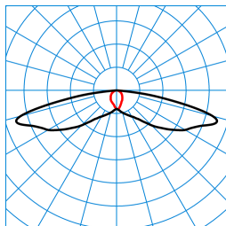
LIQ 50N-SB3L-LR-SLR2/2200-722 2G1 ET (CLO initial value) TX779392
