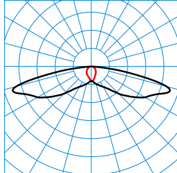
LIQ 50N-SB3L-LR-SLR2/2200-722 2G1 ET (CLO end value) TX779388
