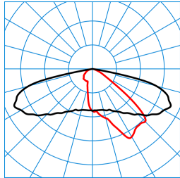
LIQ 50N-AB2L-LRA/4200-722 4G1 ETDD (CLO end value) TX778998
