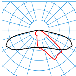
LIQ 50N-AB2L-LRA/4200-722 4G1 ETDD (CLO initial value) TX779002
