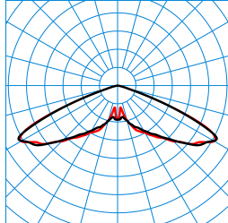
Publisca P1W-RB6L-LR/3800-740 6G1S TX053536
