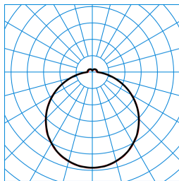
Olisq QWD3 DW 30-830 ETDD IP54 TX375733
