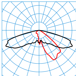
Publisca P1W-AB2L/3200-730 4G1S ETDD (CLO initial value) TX301171
