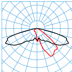
Publisca P1W-AB2L/3200-730 4G1S ETDD (CLO end value) TX301033
