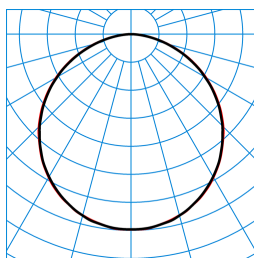
Olisq QWD3 DW 30-830 ETBLE +CAS-S IP54 + Olisq QWD3 ZDR 1/1 03 TX565506
