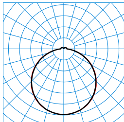
Olisq QWD3 DW 30-830 ETBLE +CAS-S IP54 + Olisq QWD3 ZDR 1/2 01 TX565517
