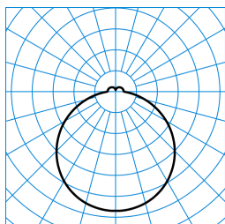
Olisq RWD2 DW 20-8TW ETBLE +CAS IP54 (DCW) TX873466
