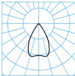
SNS RC5-MR1VFL-20-940
