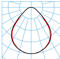
Opendo M39 PW19 42-830 ETDD TX377472
