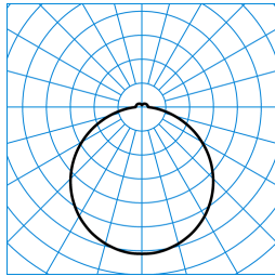
Olisq RWD4 DW 60-830 ETBLE +DMM IP54 PC TX376036
