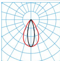
ELINE LEN55-140 ML 840 L225 0 50
