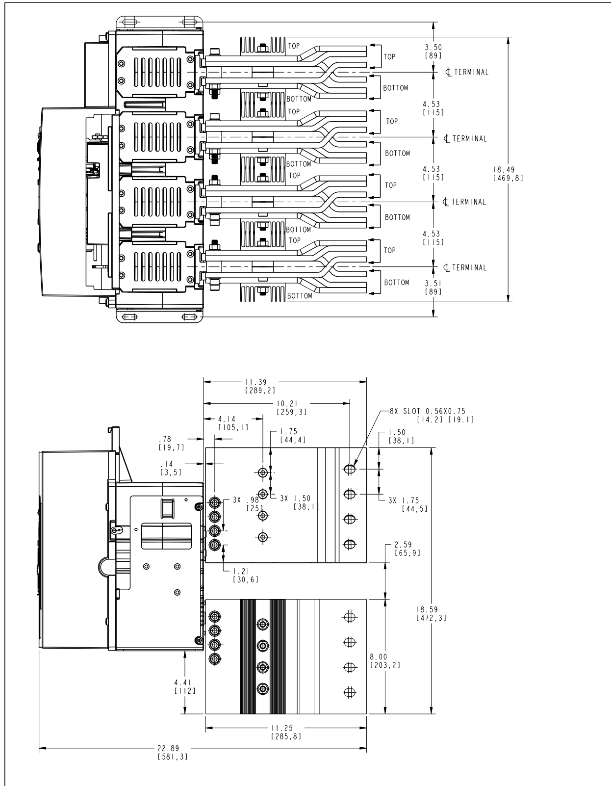
Figure 65. Four pole fixed breaker-top/side views with stamped adapter in inches (mm)-UL only.
