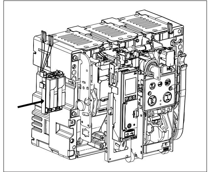
Figure 32. Right accessory tray.
