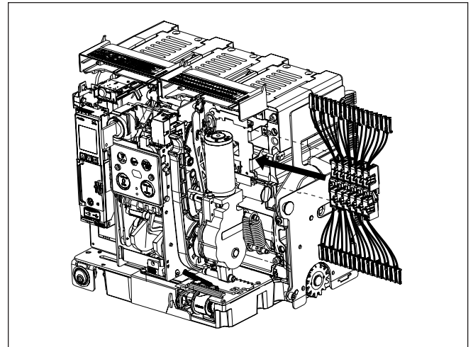
Figure 32. Right accessory tray.
