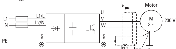
图片 10: DE1...-12...NN-N20N (不带射频干扰滤波器)
