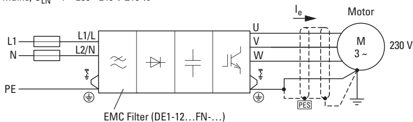
图片 9: DE1...-12...FN-N20N (带有射频干扰滤波器)
