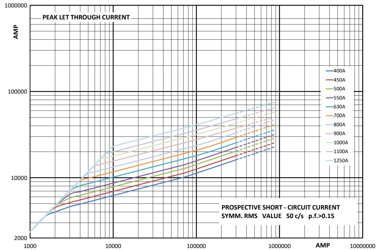
Cut-off curve - Size 2, 400 A to 1250 A
