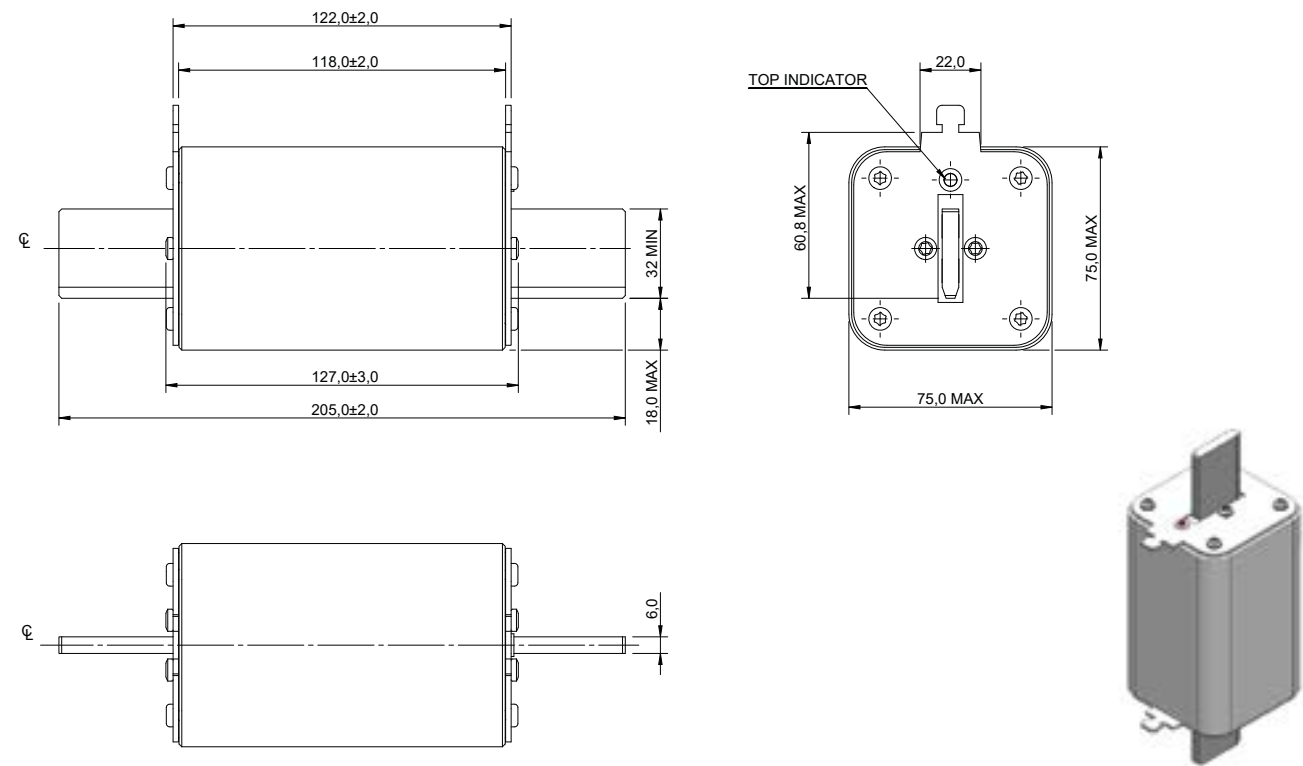
Dimensions (mm) - Size 3, bladed
