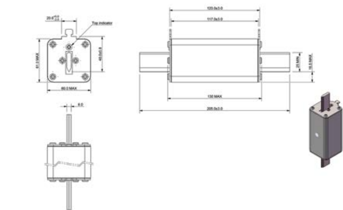
Dimensions (mm) - Size 2, bladed
