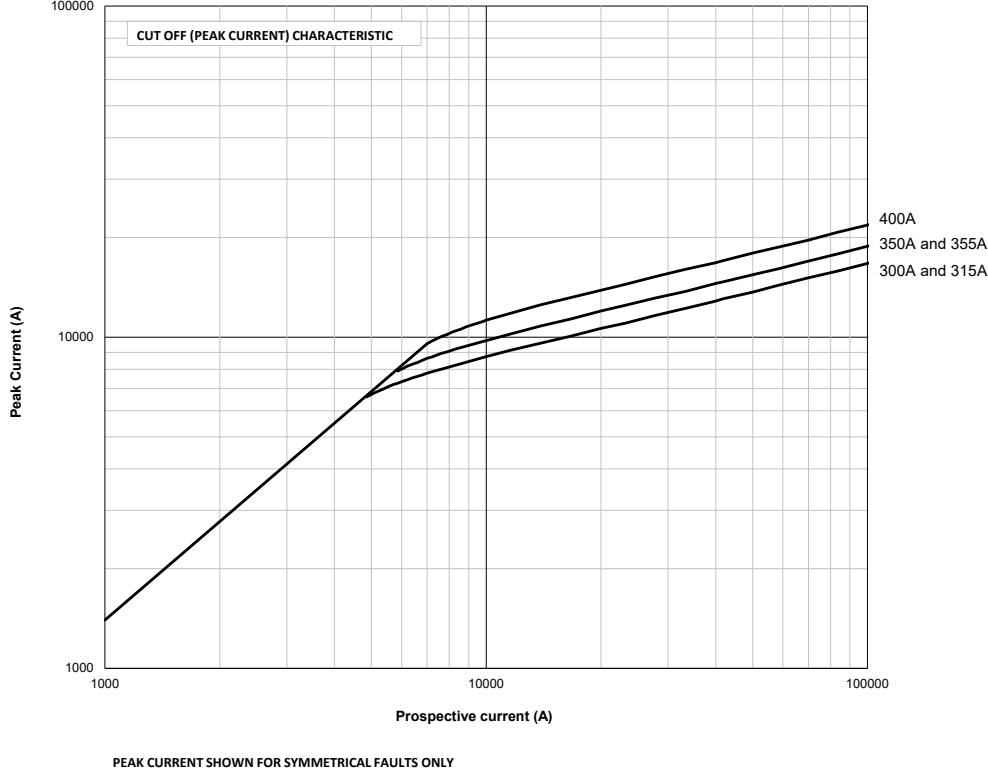
Cut-off peak current curve - Sze 3, 315 A to 400 A
