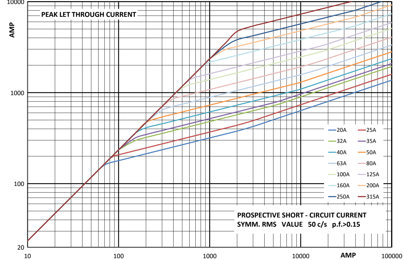
Cut-off curve - 20 A to 315 A
