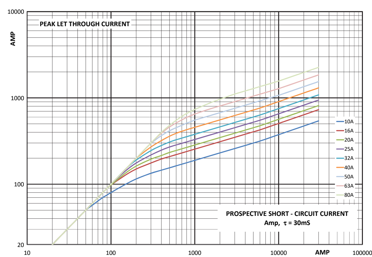
Cut-off curve - 10 A to 80 A
