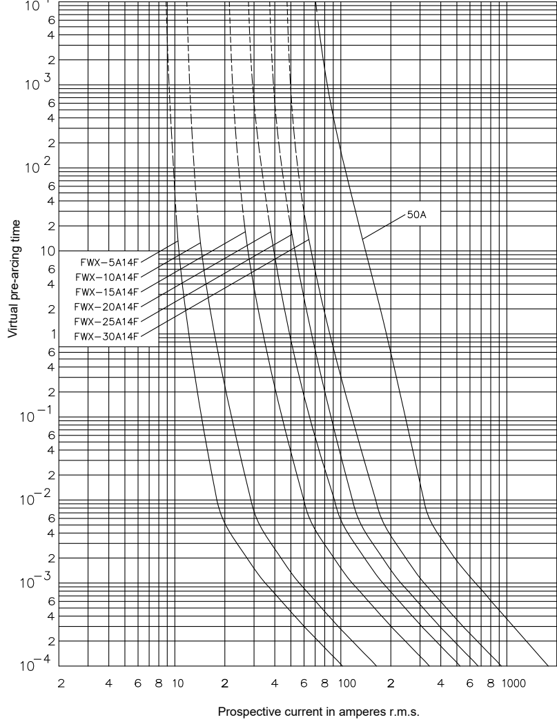
Time-current curve - 5 A to 50 A
