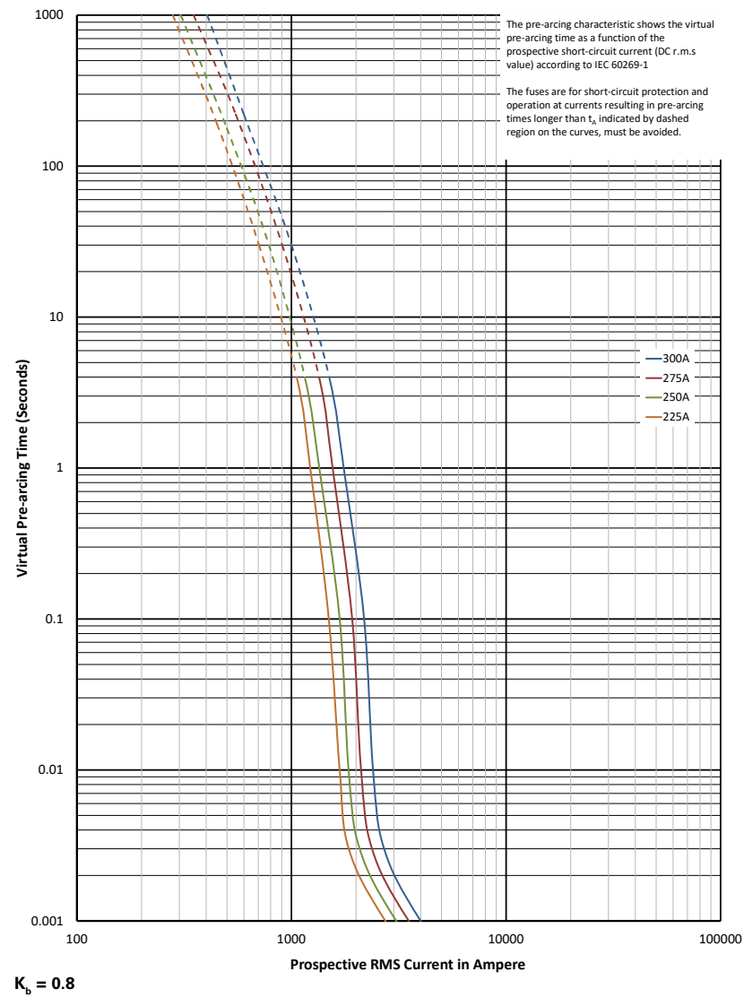
Time-current curve - 225 A to 300 A
