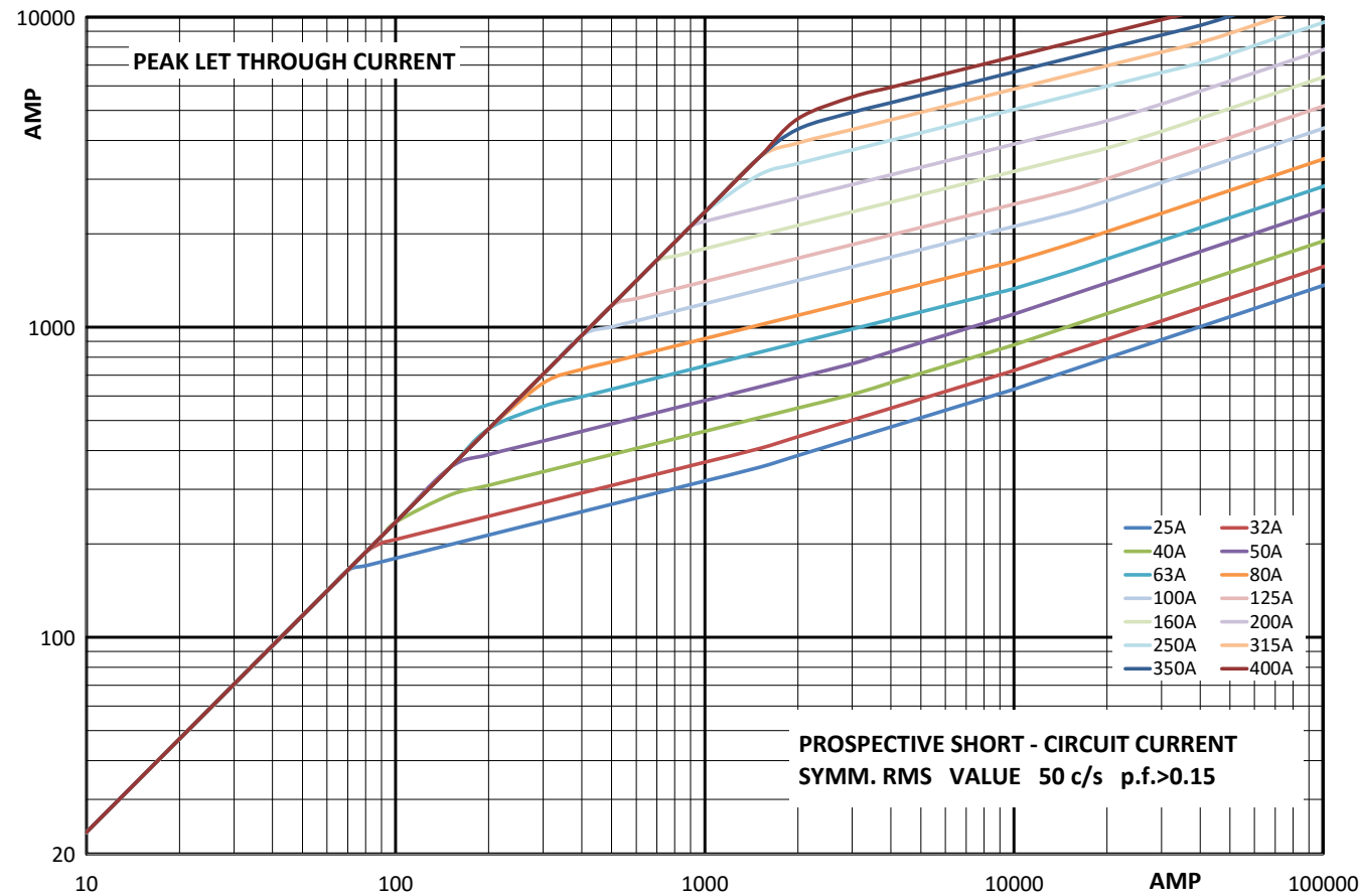
Cut-off curve- Size 00 , 25 A to 400 A
