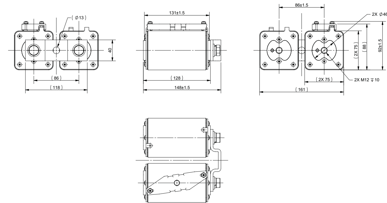
Dimensions (mm) - Size 23, 170M2017 to 170M2021, Parallel
