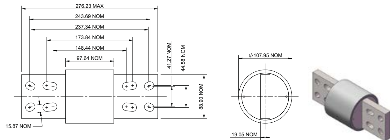
Dimensions (mm) - 1200 A
