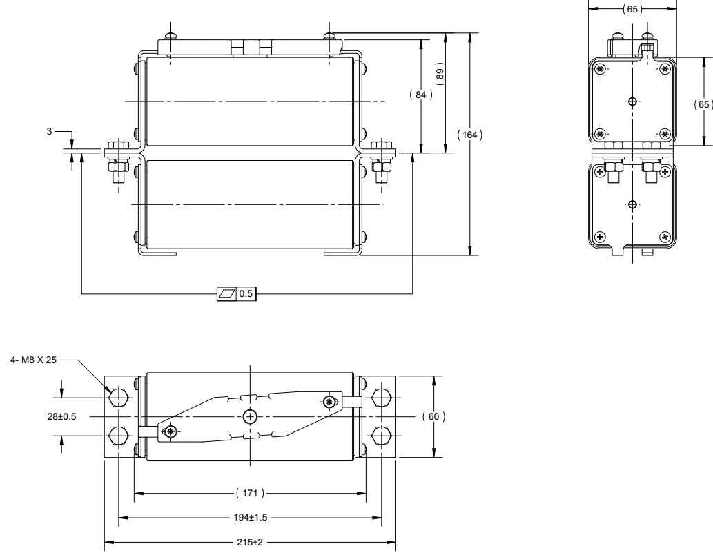
Dimensions (mm) - 170M2044 and 170M2045, Parallel, double slot tag
