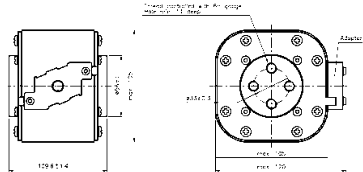
Dimensions (mm) - 4BKN/110
