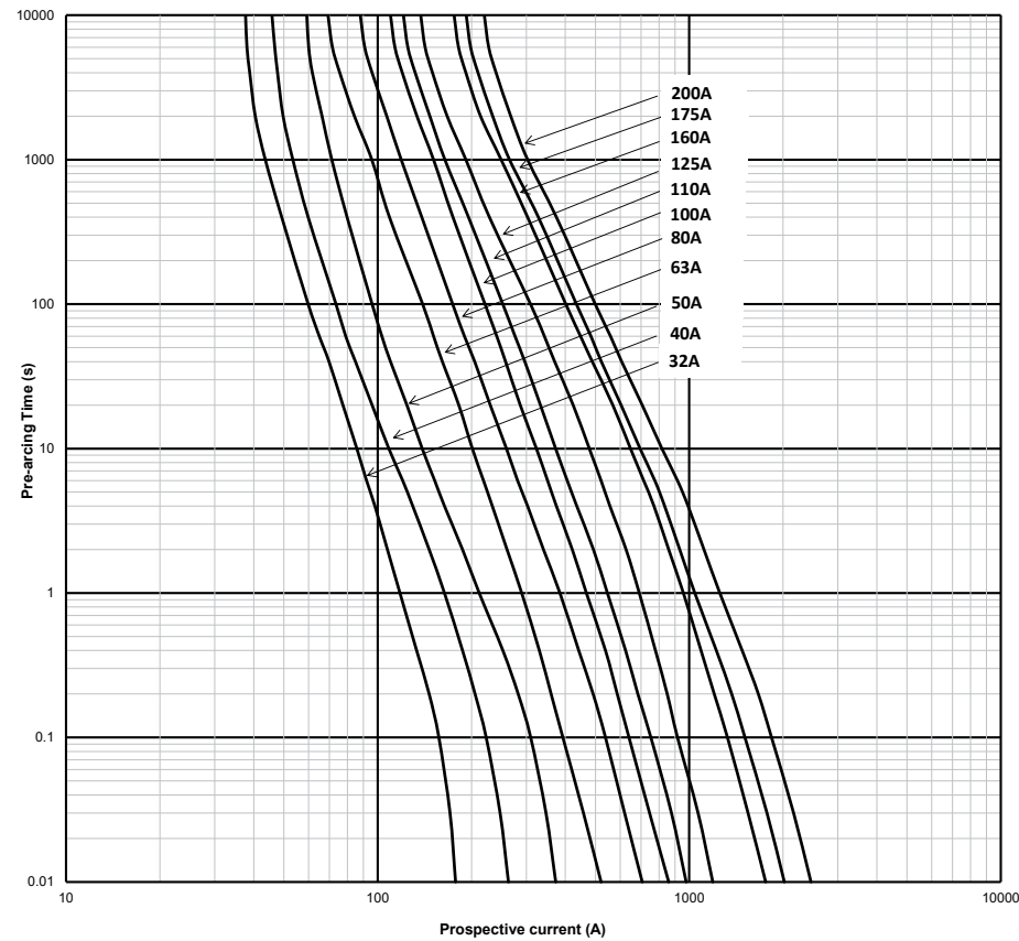
Time-current curve - Size 1, 32 A to 200 A
