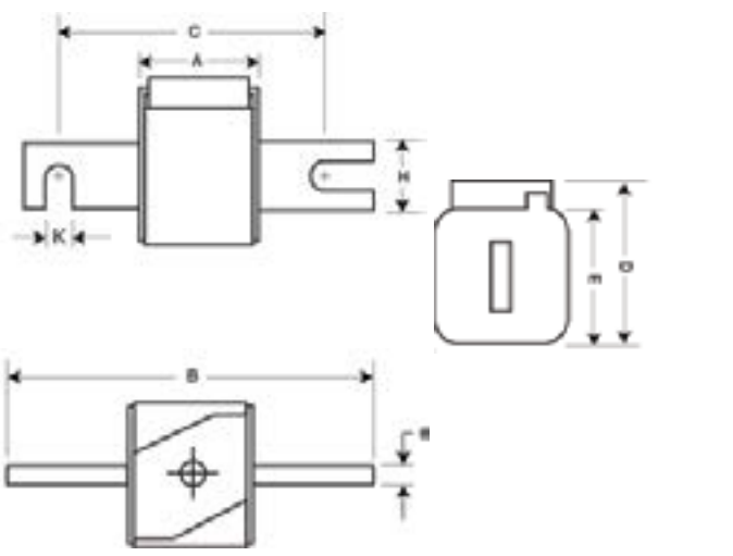
Dimensions (mm) - KN/110
