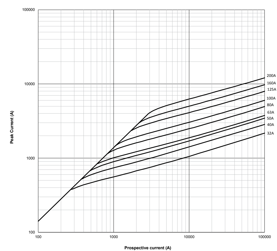
Cut-off curve - Size 1, 32 A to 200 A
