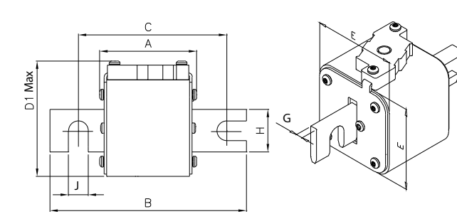
Dimensions (mm) -KN/110
