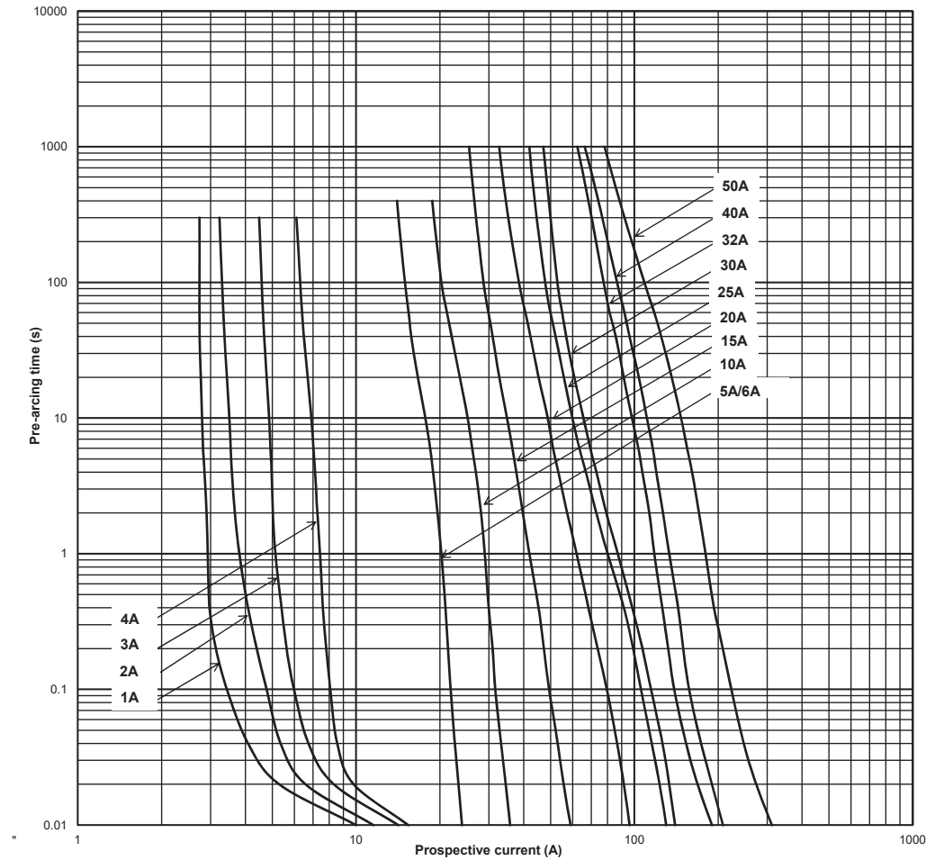
Time-current curve - 1 A to 50 A
