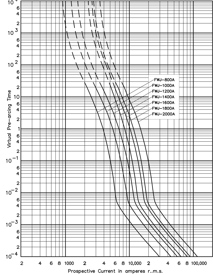
Time-current curve - 800 A to 2000 A
