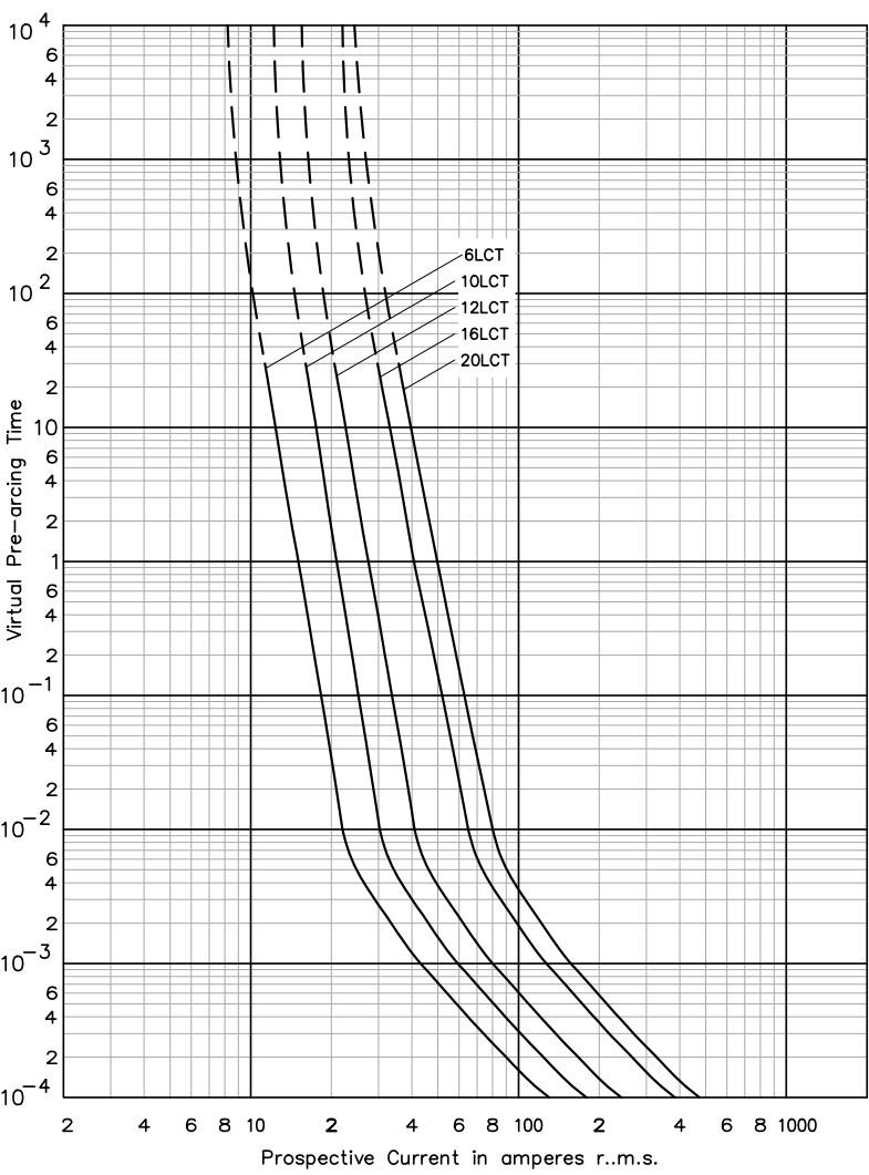
Time-current curve - LCT, 6 A to 20 A
