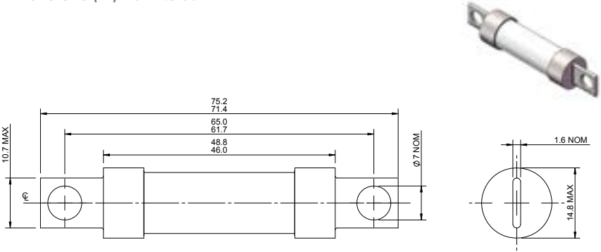
Dimensions (in) - 5 A to 30 A
