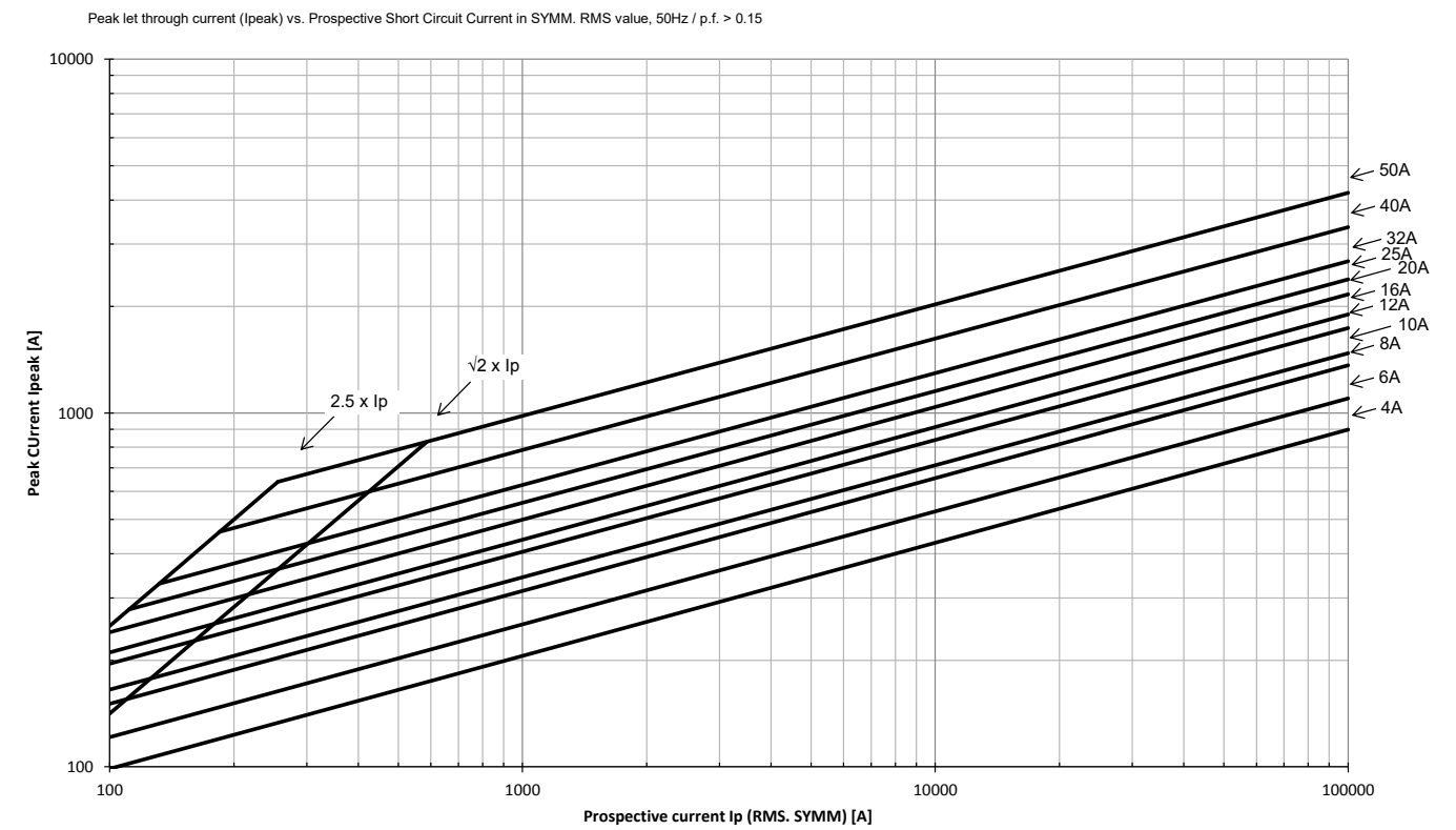
Cut-off curve - 4 A to 50 A
