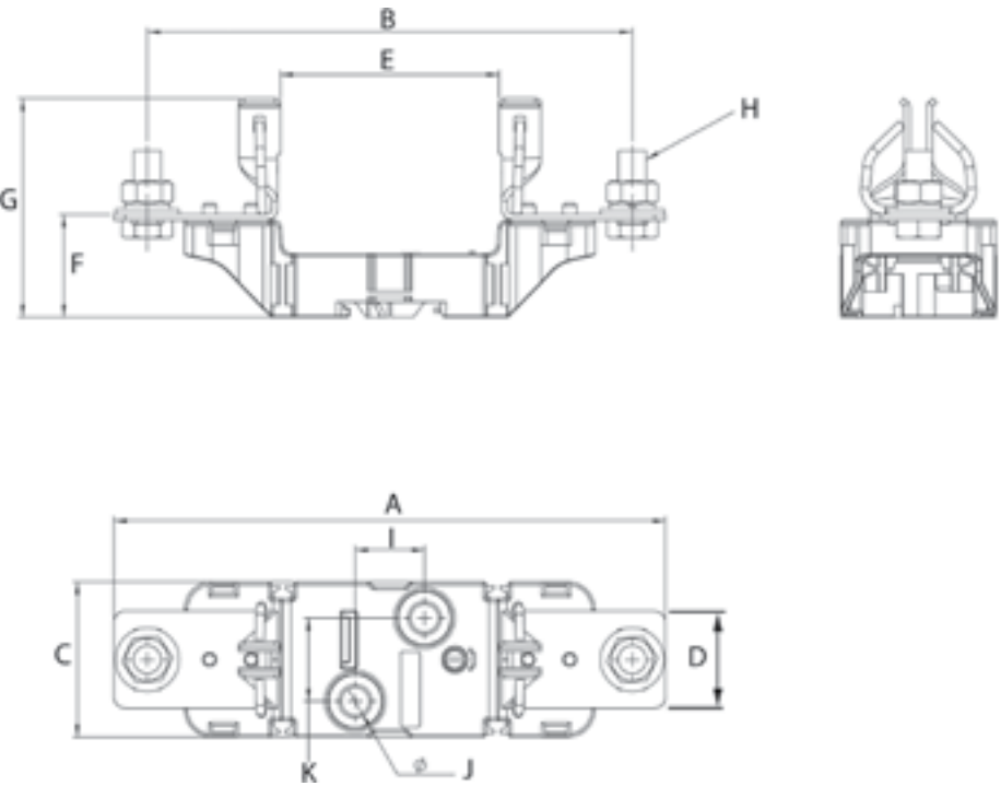
Dimensions (mm) - 1-pole without phase barriers
