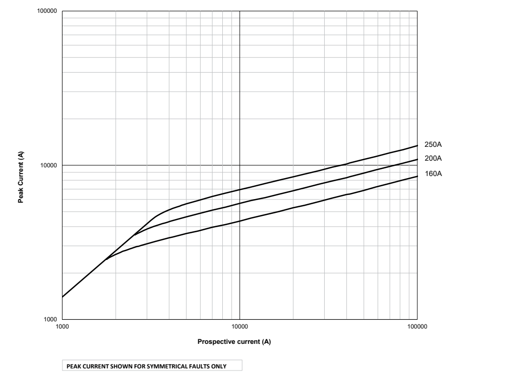
Cut-off curve - Size 2, 160 A to 250 A
