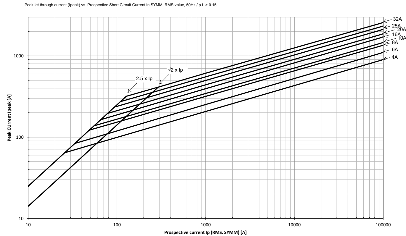
Cut-off curve- 2 A to 32 A
