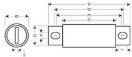
Dimensions (in) - 70 A to 600 A
