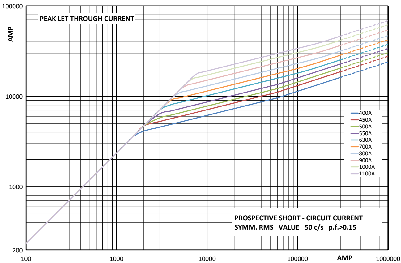
Cut-off curve - Size 2, 400 A to 1100 A
