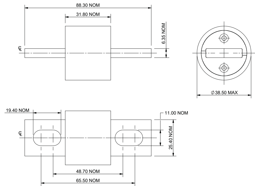
Dimensions (mm) - 500 A to 1000 A
