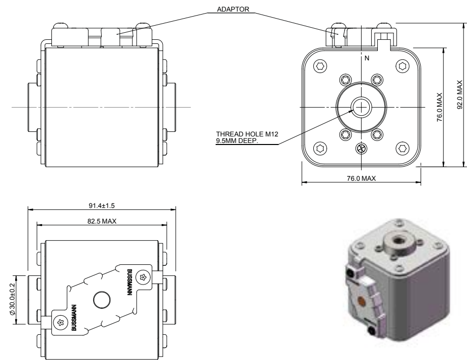
Dimensions (mm) - Size 3
