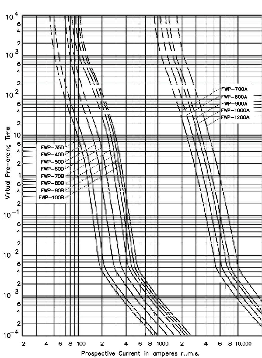
Time-current curve - 35 A to 1200 A
