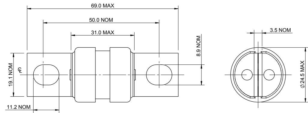
Dimensions (mm) - 70 A to 400 A
