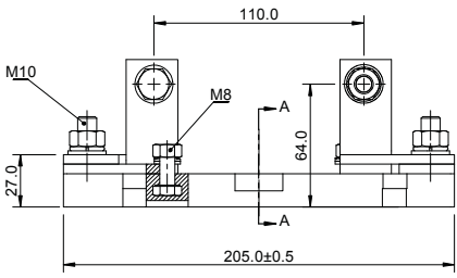
Dimensions (mm) - 170H3006
