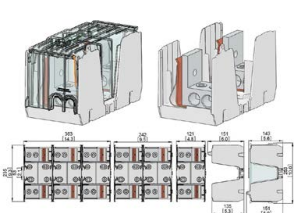
Dimensions mm (in) - 600 A
