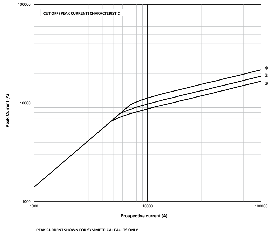
Cut-off curve - Size 3, 300 A to 400 A
