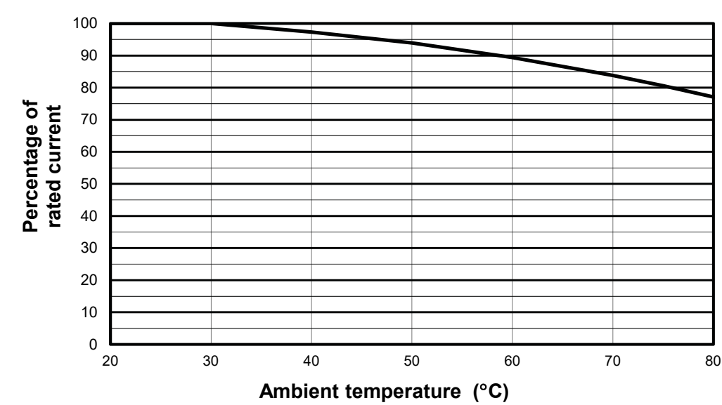
Temperature derating
