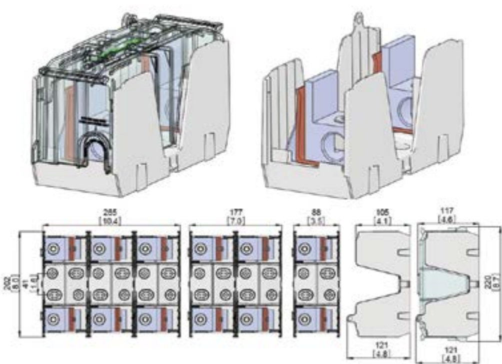
Dimensions mm (in) - 400 A
