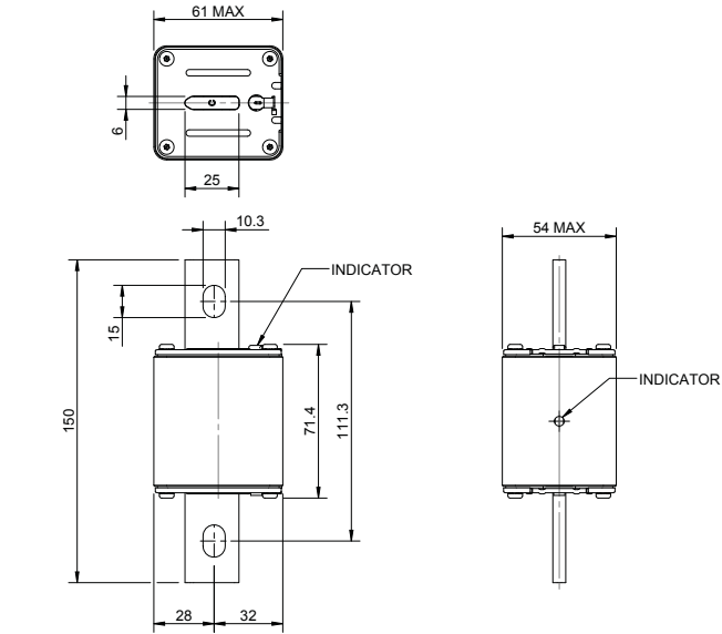
Dimensions (mm) - NH2, bolt holes no lugs
