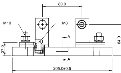
Dimensions (mm) - 170H3004
