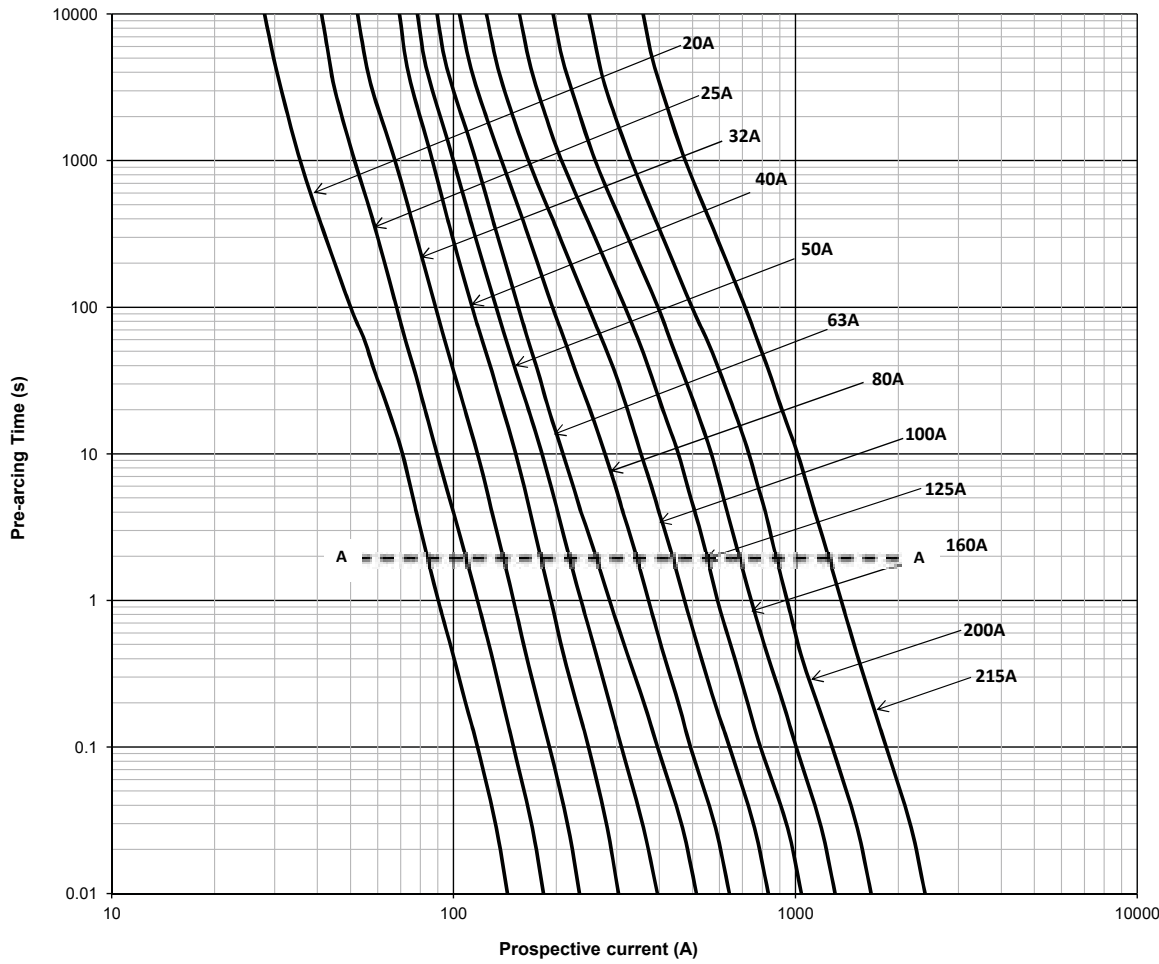
Time-current curve - 170M2046 to 170M2056, 20 A to 215 A
