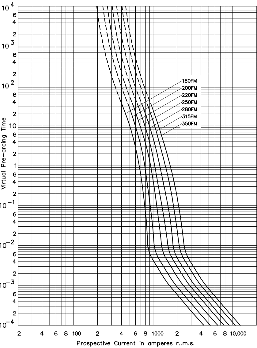
Time-current curve - FM, 180 A to 350 A
