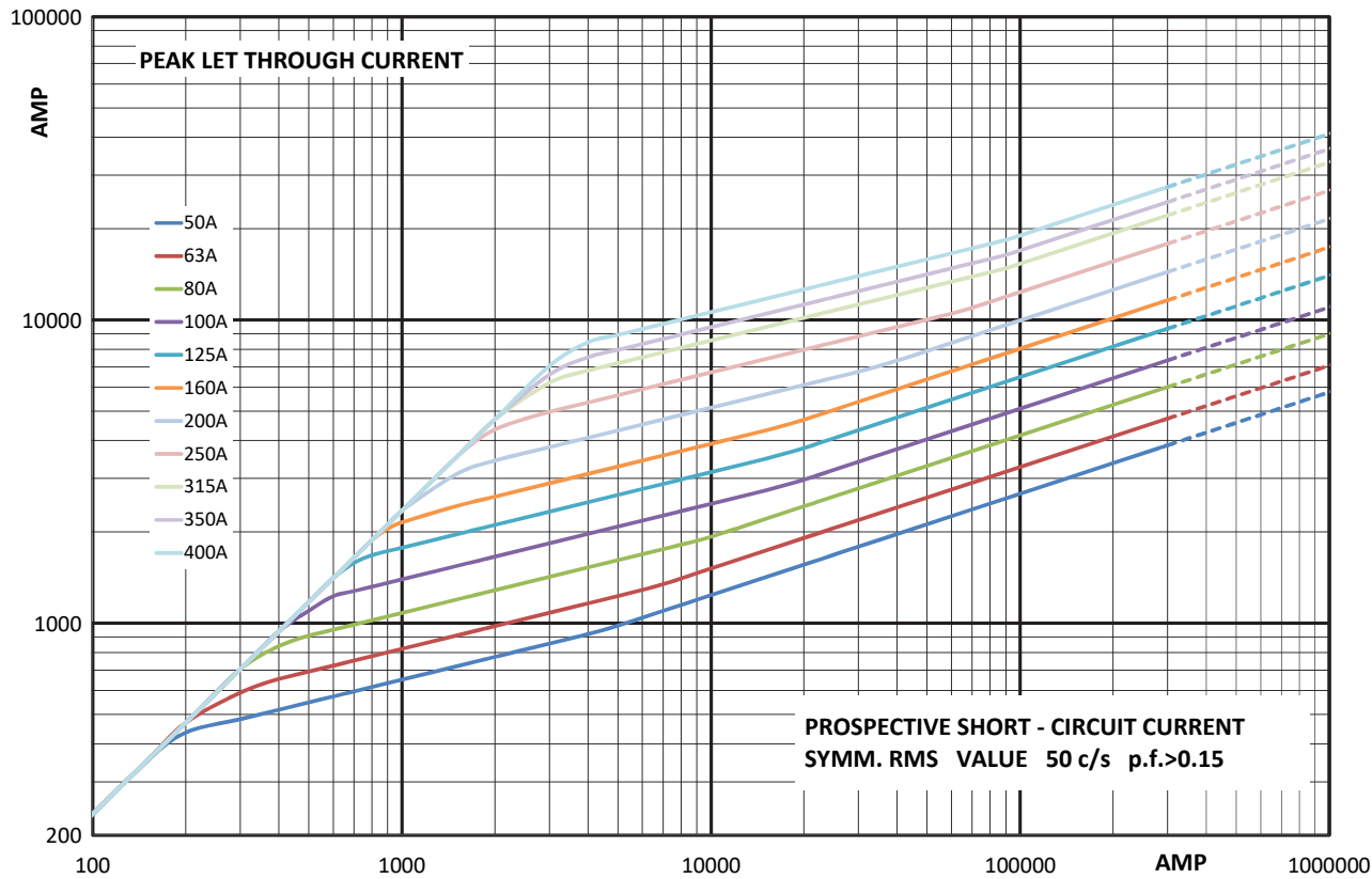
Cut-off curve - Size 1, 50 A to 400 A
