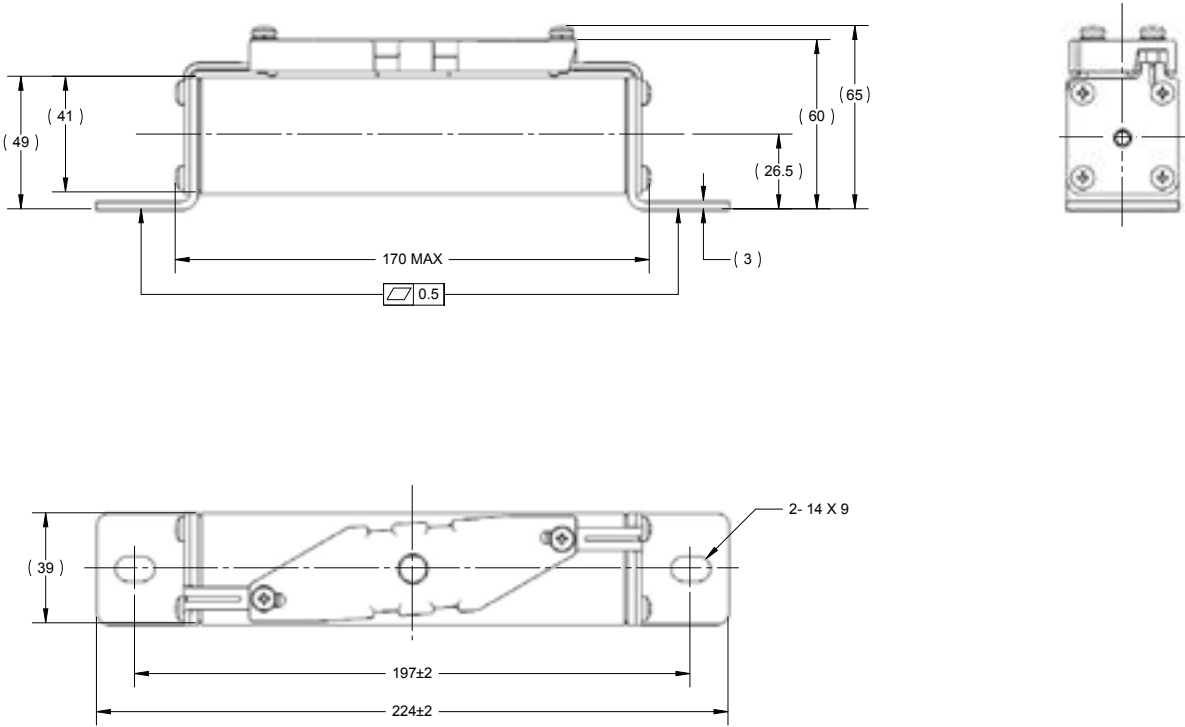
Dimensions (mm) - 170M2039 to 170M2043, Double slot tag
