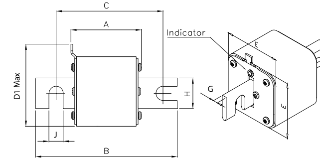
Dimensions (mm) -TN/110
