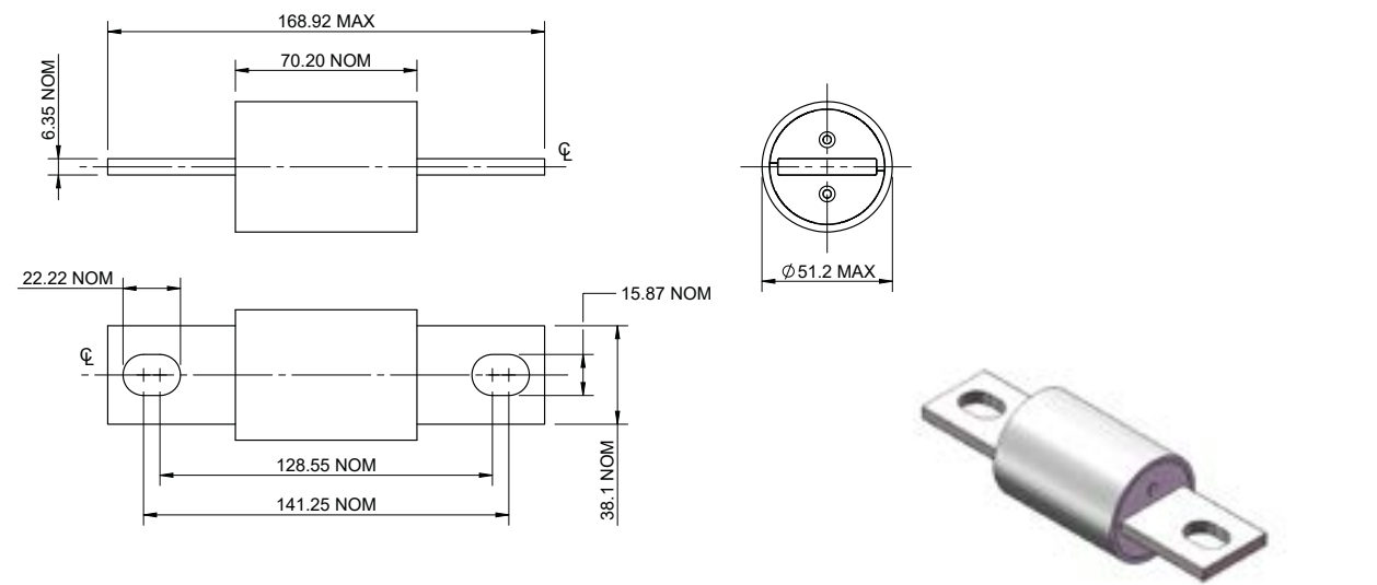
Dimensions (in) - 700 A and 800 A
