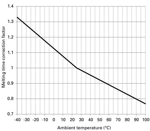
Temperature derating
