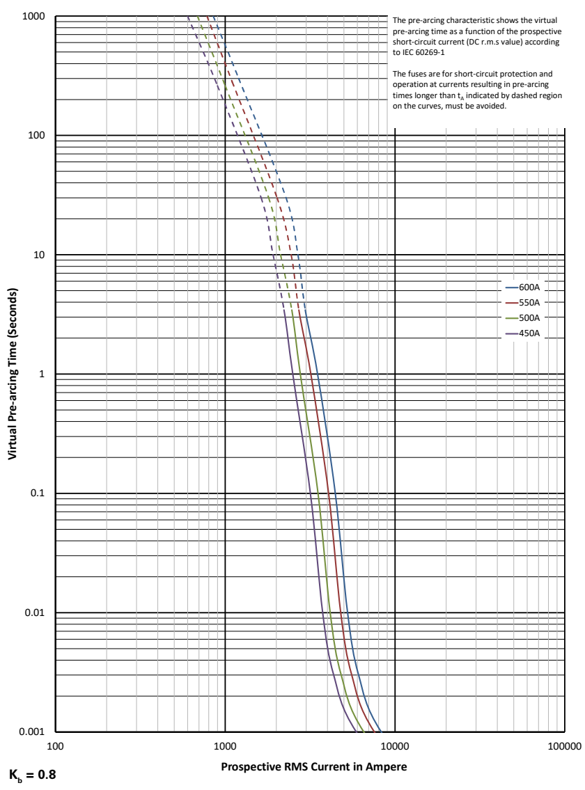
Time-current curve - 450 A to 600 A
