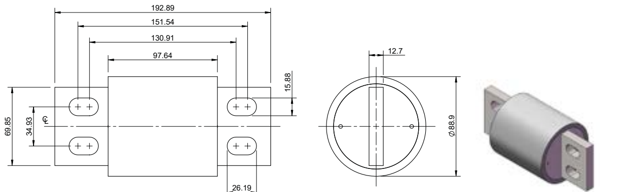
Dimensions (mm) - 1200 A
