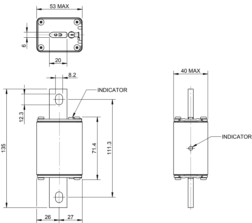
Dimensions (mm) - NH1, blade with bolt holes
