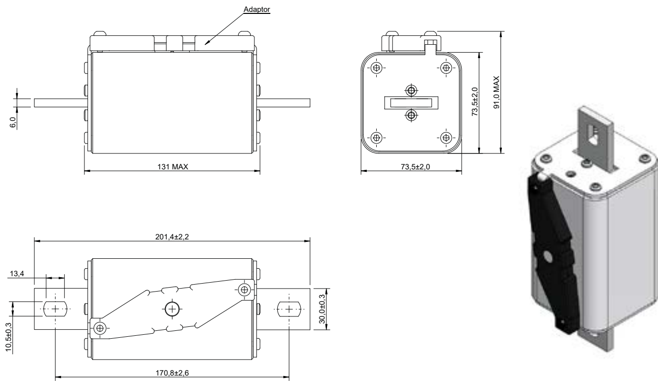
Dimensions (mm) - Size 3, bolted
