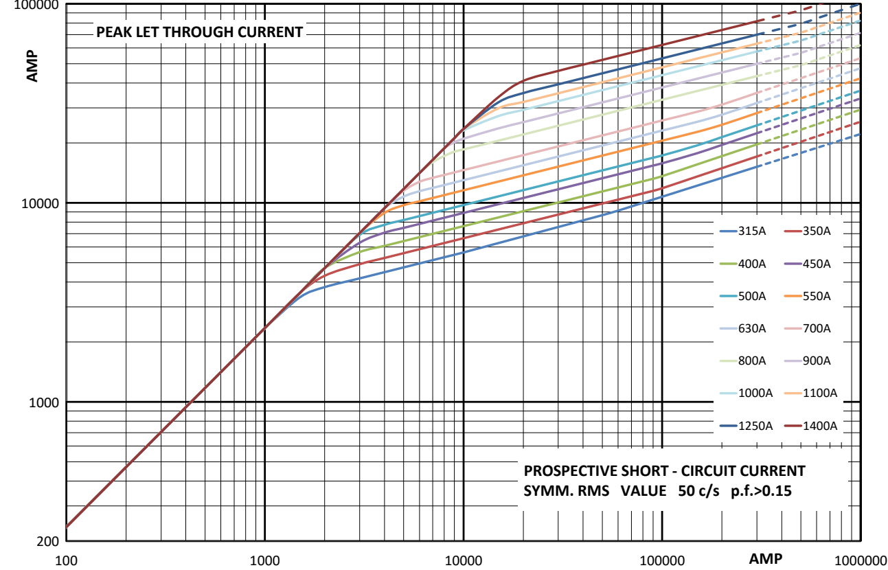
Cut-off curve - Size 3, 315 A to 1400 A
