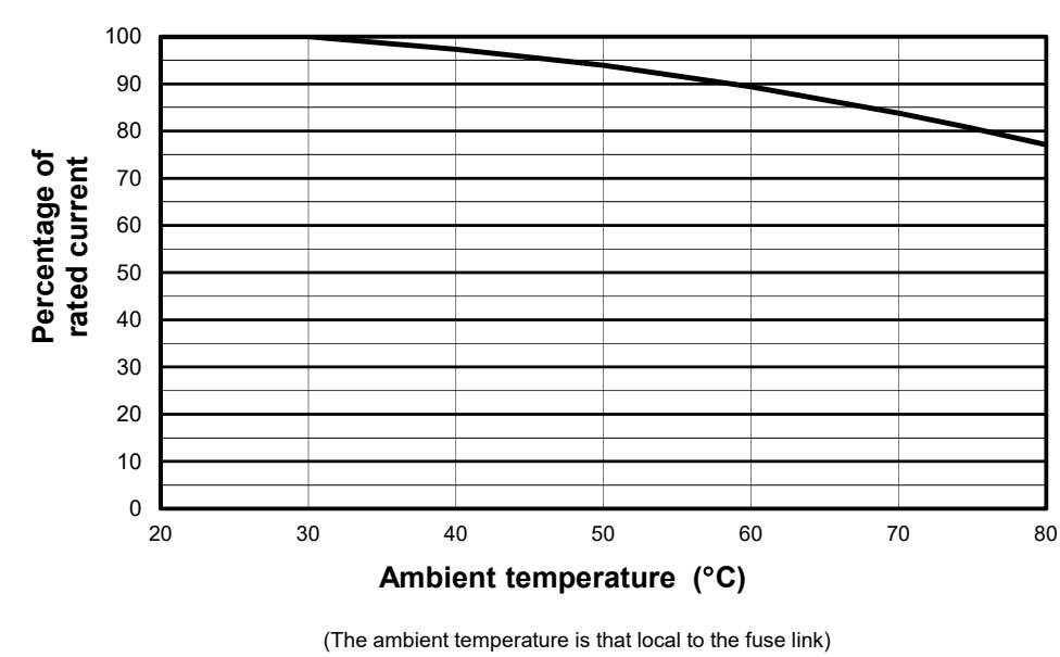
Temperature derating
