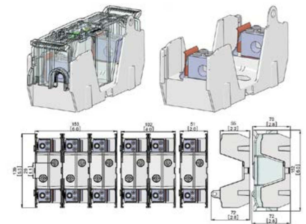
Dimensions mm (in) - 100 A
