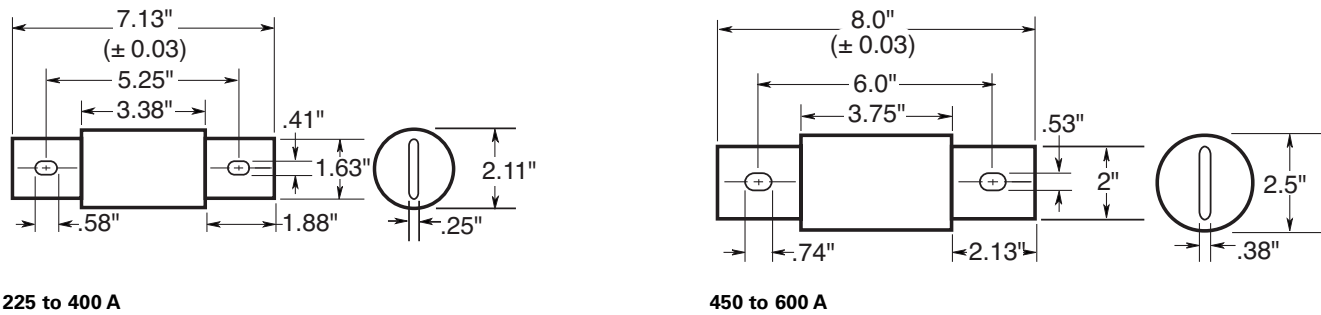
Dimensions (in)
