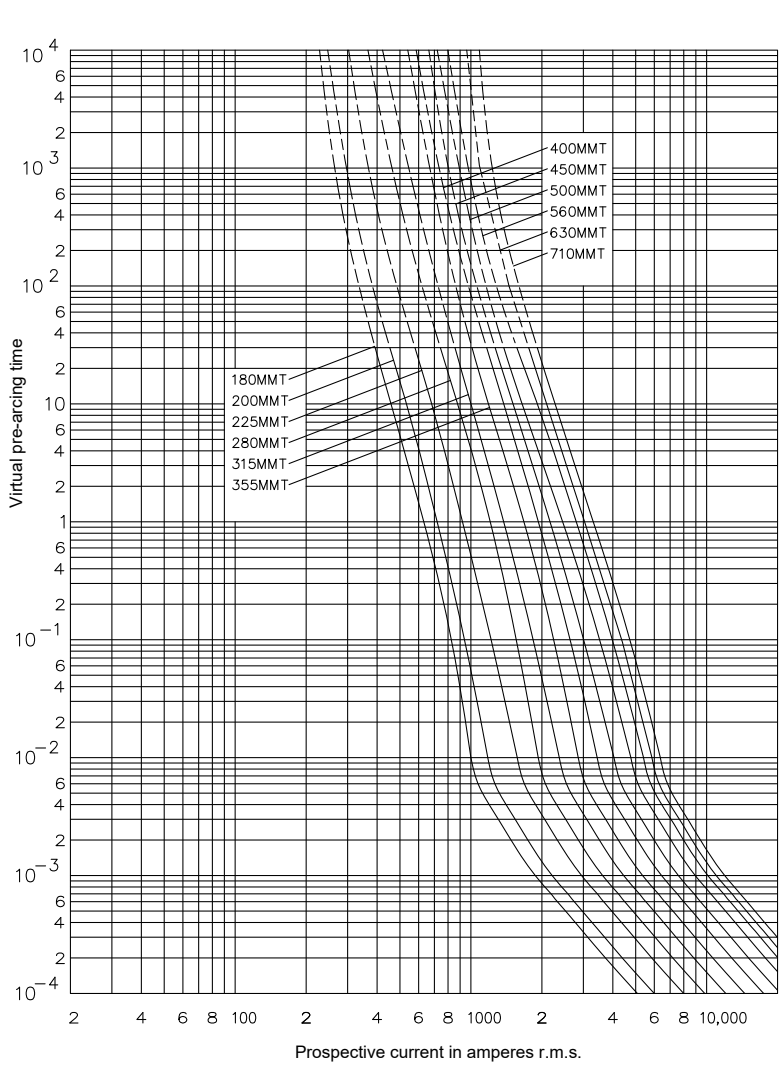
Time-current curve - MMT, 180 A to 710 A
