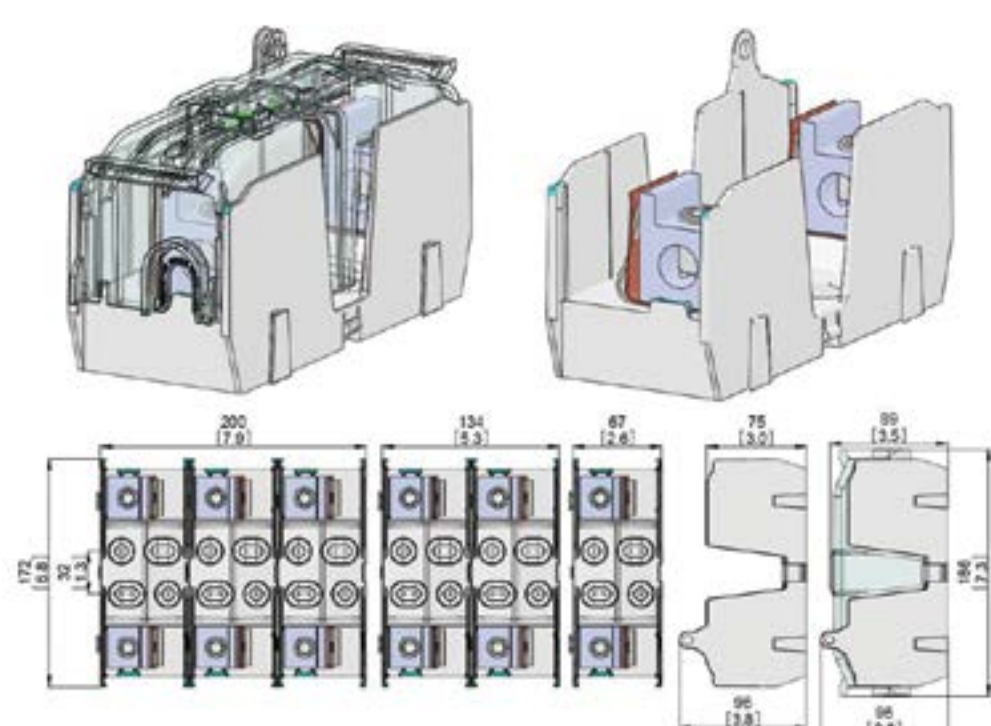
Dimensions mm (in) - 200 A
