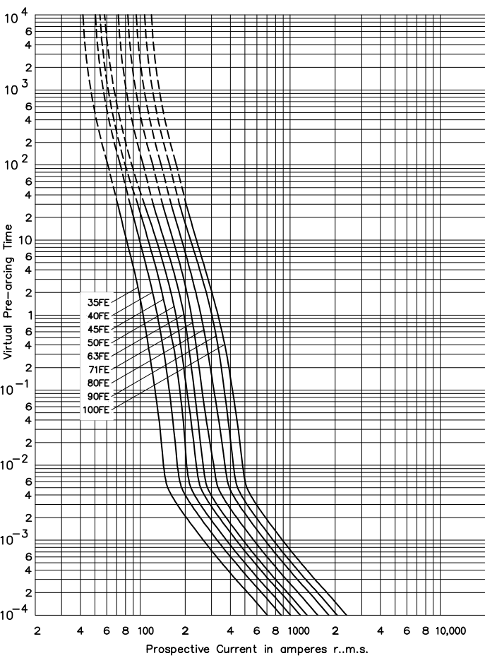
Time-current curve - FE, 35 A to 100 A
