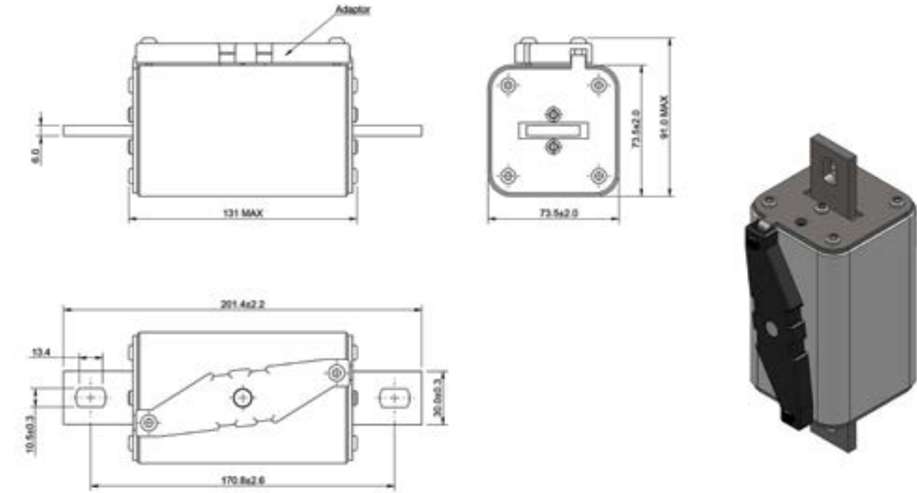
Dimensions (mm) - Size 3, bolted
