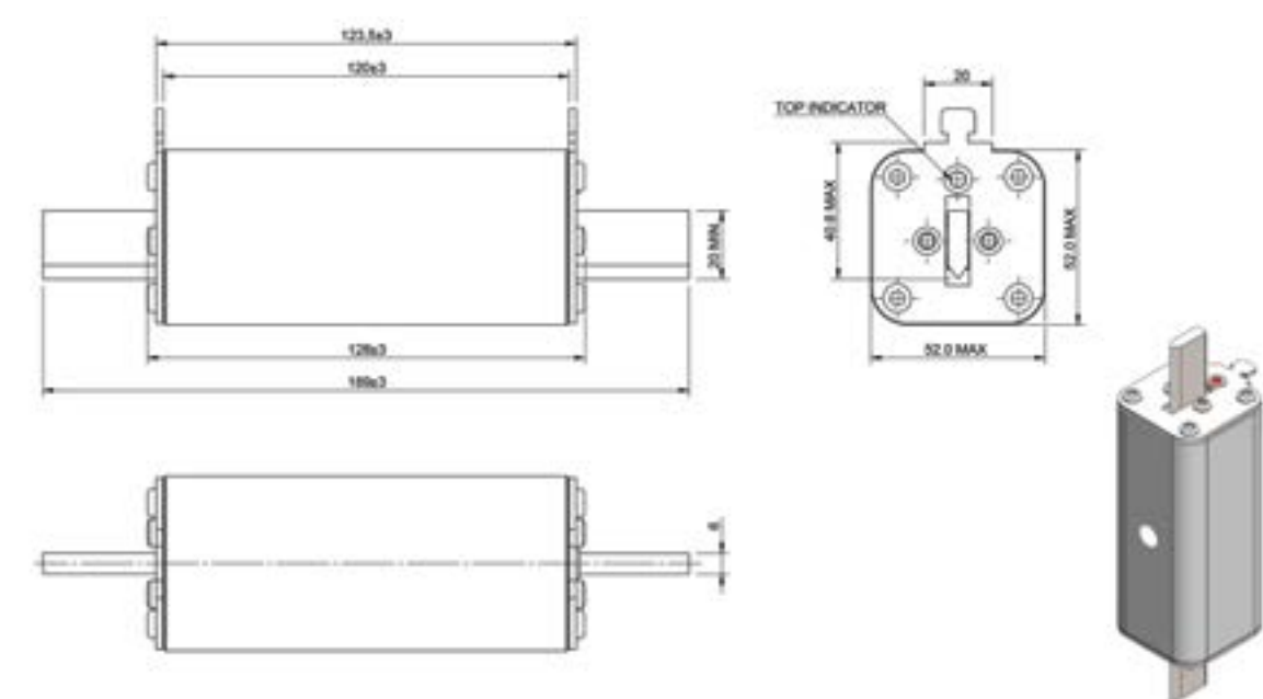
Dimensions (mm) - Size 1, bladed
