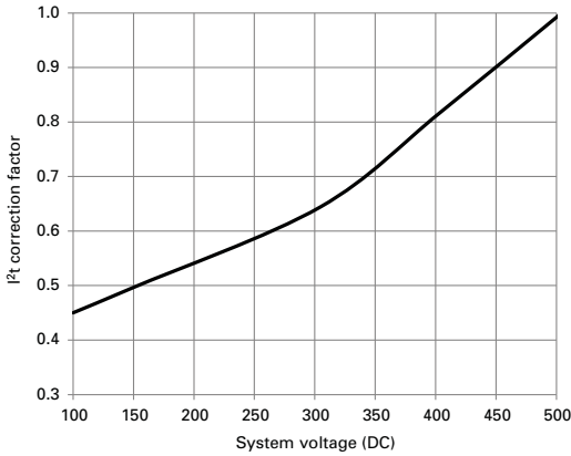
DC clearing I²t voltage correction factor
