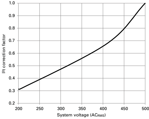
AC clearing I²t voltage correction factor
