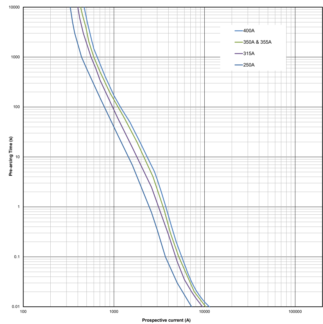
Time-current curve
