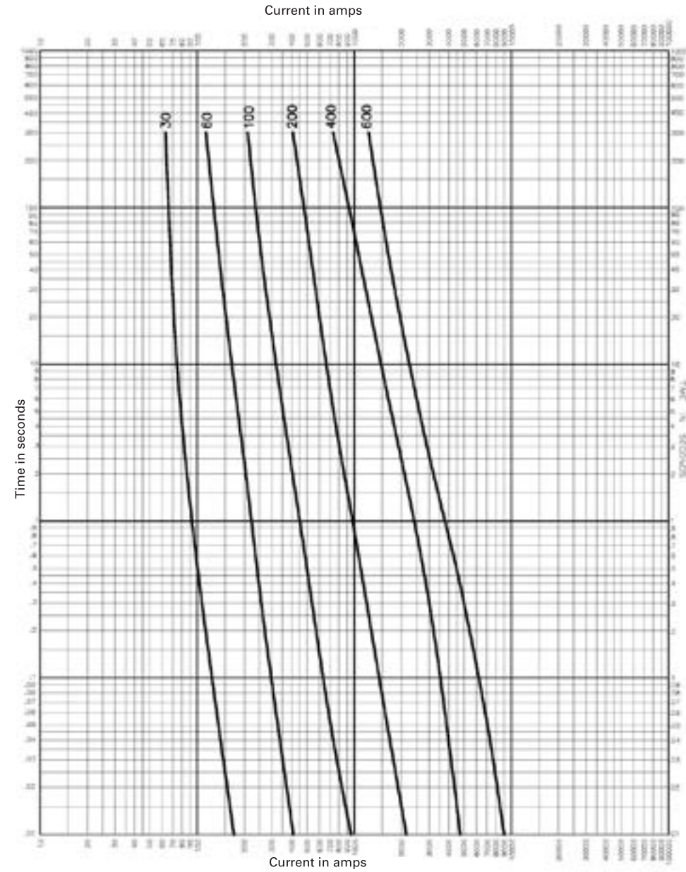
Time-current curve - 30 A to 600 A
