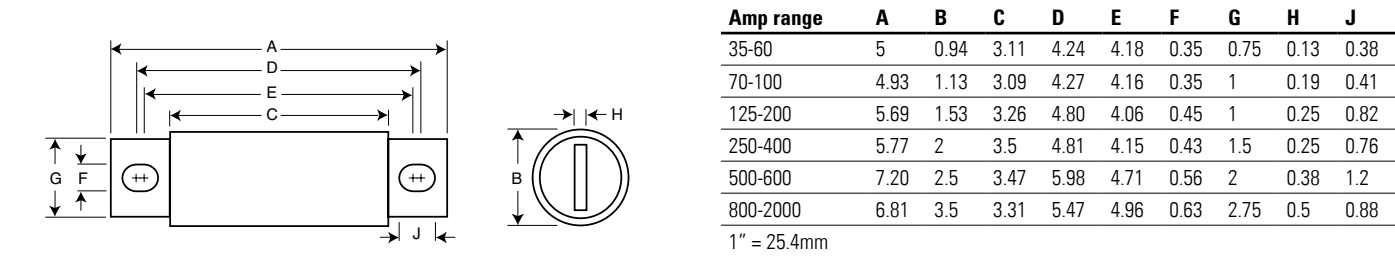
Dimensions (in) - 35 A to 2000 A
