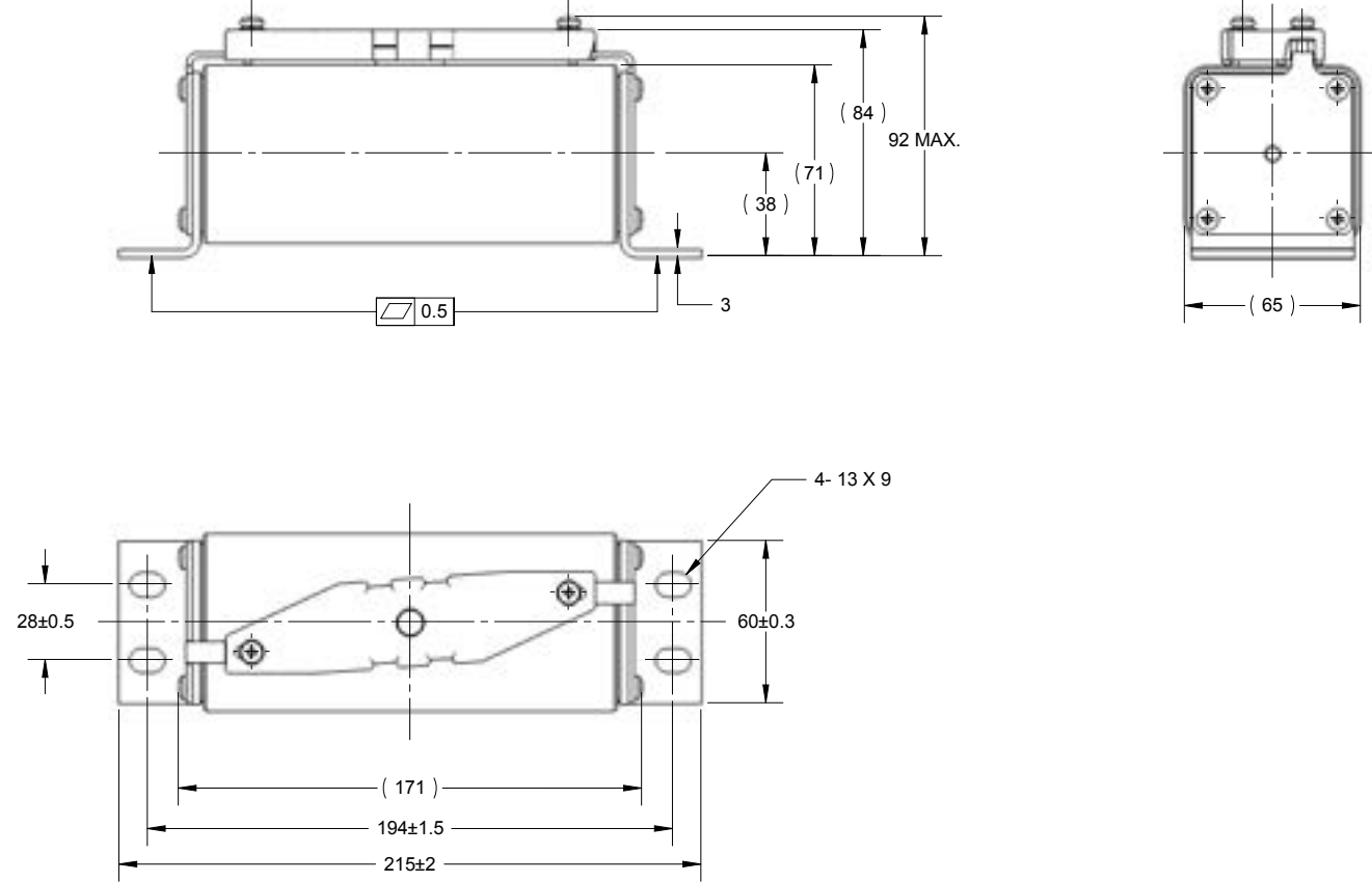
Dimensions (mm) - 170M2039 to 170M2043, Double slot tag
