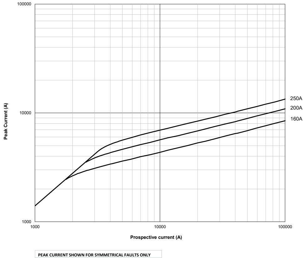
Cut-off peak current curve - Size 2, 160 A to 250 A
