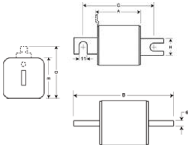
Dimensions (mm) -110 and TN/110
