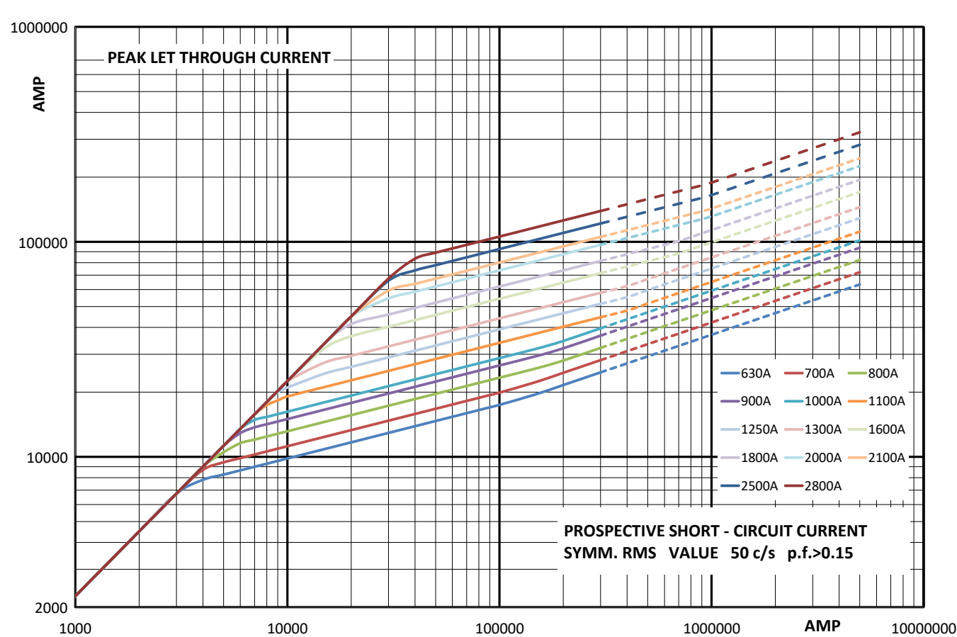
Cut-off curve - 630 A to 2800 A
