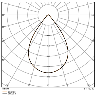
HB P 173W 865 70DEG IP66 PS
