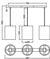
DECOR CARDBOARD CYLINDER PEND 3XE27
