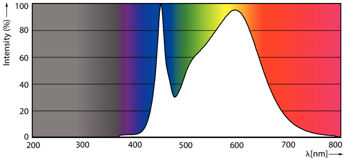
Spectral Power Distribution Colour - CorePro LED Urban PLL Mains 13W 840
