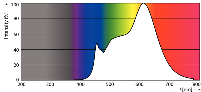
Spectral Power Distribution Colour - MAS LEDspot VLE D 6-50W 930 PAR20 40D
