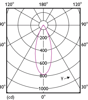
Light Distribution Diagram - MAS LEDspot UE 2.4-50W GU10 ND 840 EELB
