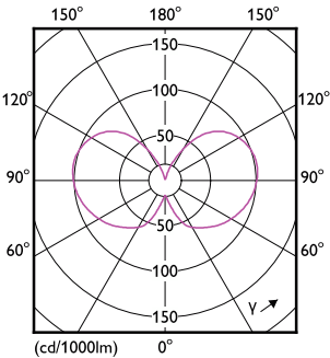
Light Distribution Diagram - MAS LEDBulbND2.3-40W E27 840 A60 CL G UE
