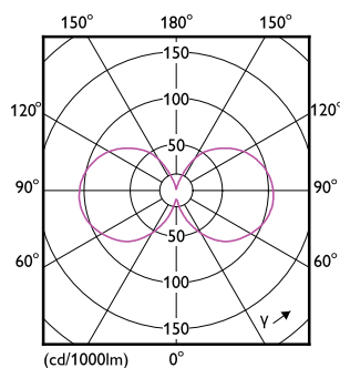
Light Distribution Diagram - MAS LEDBulbND2.3-40W E27 830 A60 FR G UE
