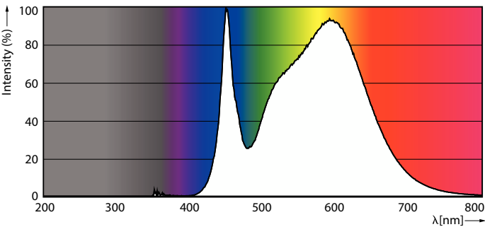
Spectral Power Distribution Colour - CorePro LED HPI MV 15Klm 105W840E40 100D
