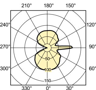
Light Distribution Diagram - MASTERColour CDM-T 35W/842 G12 1CT/12
