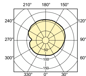
Light Distribution Diagram - MASTERColour CDM-T 35W/842 G12 1CT/12
