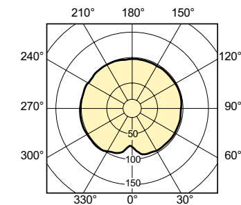
Light Distribution Diagram - MASTERColour CDM-T 35W/842 G12 1CT/12
