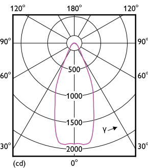
Light Distribution Diagram - MAS LEDExpertColor 20-100W 930 AR111 45D
