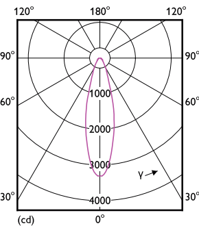
Light Distribution Diagram - MAS LEDExpertColor 20-100W 940 AR111 24D
