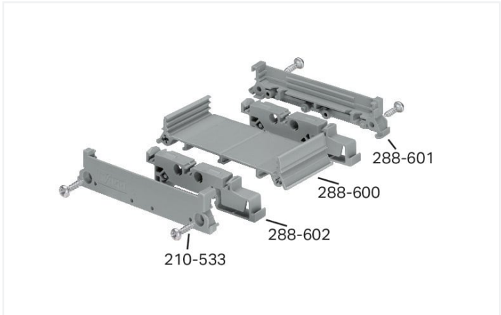
DIN-rail-mount PCB carrier, size 1
