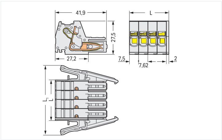
Dimensions in mm L = (\text{pole no.} - 1) \times \text{pin spacing} + 10.5 \text{ mm} L1 = L + 23.7 \text{ mm}
