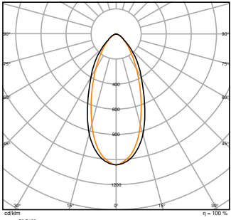
OFFICE LINEAR V 2CCT UGR19 29W 4000K
