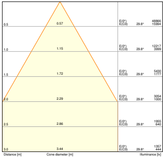
HB DA P 75W 865 110DEG IP66 WITH REFLECTOR
