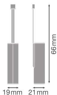
BLKH CBO RD BAT 3.2V 1.8AH 5.8WH
