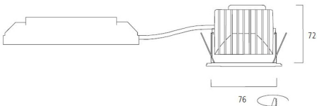
Dimensions (mm)
