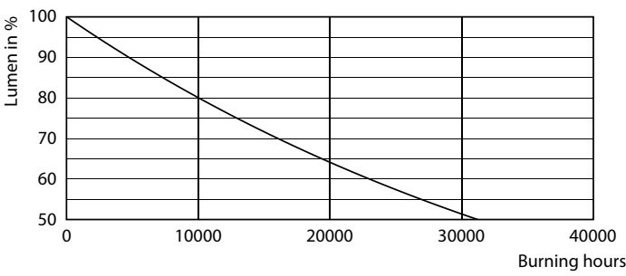
Lumen Maintenance Diagram - MAS VLE LEDBulbD3.4-40W E27 927 A60 CL G
