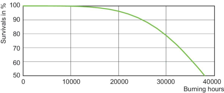
Life Expectancy Diagram - MST SON-T APIA Plus Xtra 50W E27 1SL/12
