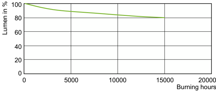
Lumen Maintenance Diagram - MC CDM-R Elite 35W/930 E27 PAR30L 30D
